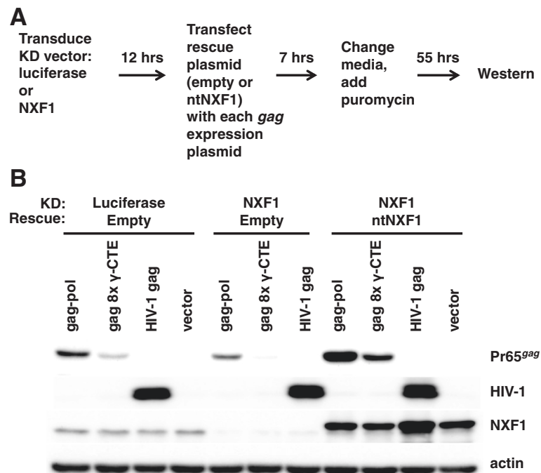
Figure 10 The effect of NXF1 KD on Pr65 Gag protein production. (A) Diagram showing protocol for short-term selection of cells with NXF1 KD. HEK293 cells were transduced with lentiviral vectors bearing miR30 frameworks targeting either luciferase or NXF1. Then, cells were transfected with the indicated plasmids, and finally selected in pools with puromycin. (B) 55 hrs after addition of puromycin cell lysate was probed by western blot with anti-gammaretrovirus CA antibody, anti-HIV-1 CA antibody, anti-NXF1 antibody, or anti-β-actin antibody, as indicated. Similar results were obtained with identical constructs from MLV and XMRV. A representative experiment with MLV derived constructs is shown.
