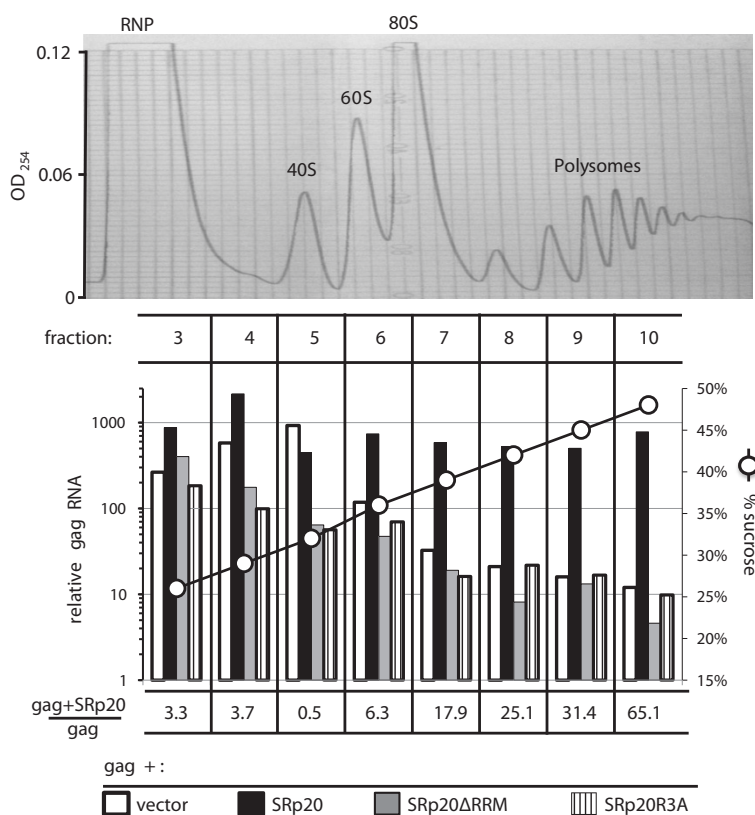
Figure 12 SRp20 promotes gag mRNA association with polysomes in an NXF1-dependent manner. HEK293T cells were transfected with expression plasmids for gag and either SRp20 wild-type, SRp20 \Delta RRM, or SRp20R3A. 48 h post-transfection cell lysate was loaded onto a 15% to 55% linear sucrose gradient. After acceleration for 3 hrs at 210,000 \times g , RNA content across the gradient was assessed by reading absorbance at 254 nm (upper panel). The position of migration of the various ribosomal components and polysomes is indicated. Fractions were collected from the gradient (lower panel) and relative gag mRNA in fractions 3 to 10 was quantified by qRT-PCR using GAPDH as a control (left Y axis) and displayed against the percent sucrose (right Y axis). The ratio of gag RNA signal expressed in the presence of SRp20 wild-type, versus the gag RNA signal in the absence of SRp20 plasmid is shown for each fraction. This experiment was repeated on three separate occasions with the same result. Similar results were obtained with identical constructs from MLV and XMRV. A representative experiment with MLV-derived constructs is shown.
